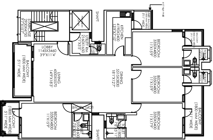
SECOND FLOOR PLAN SALEABLE AREA 2438 SQ.FT. (226.450 SQM.)
