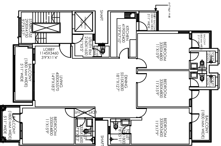
FIRST FLOOR PLAN SALEABLE AREA 2438 SQ.FT. (226.450 SQM.)
